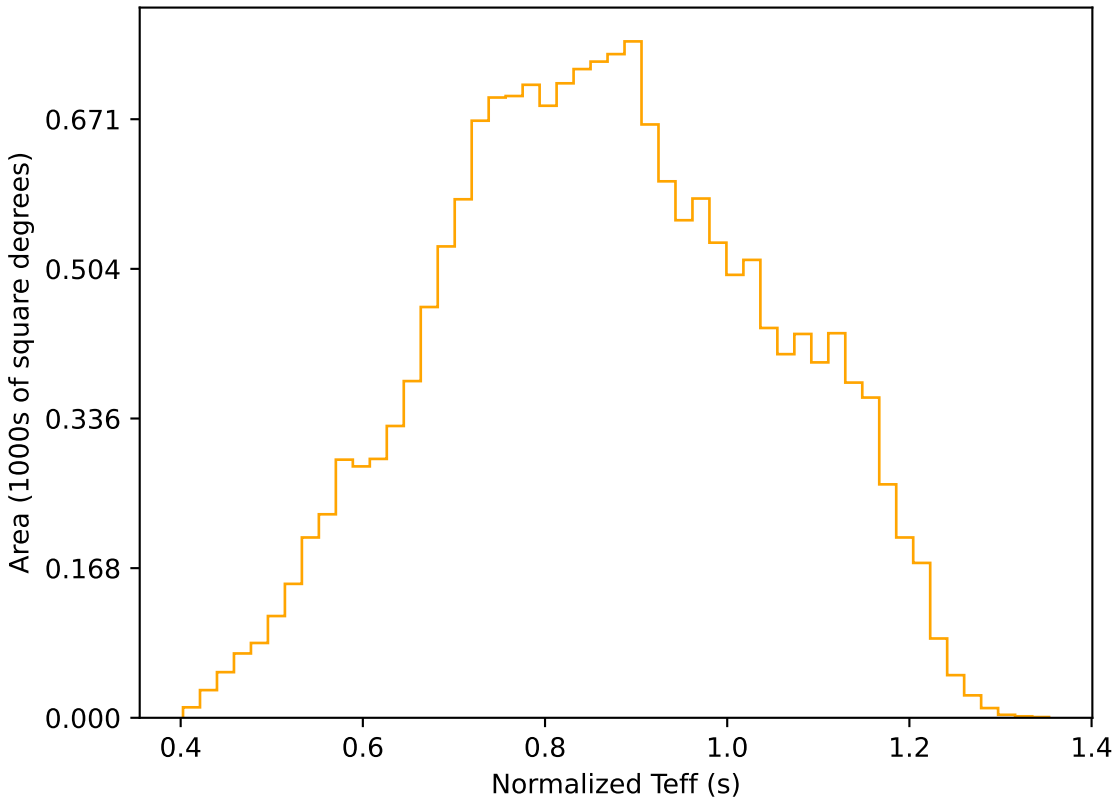
too_elab_r8_d2_giz_v3.4_10yrs WFD r band: Normalized Teff
