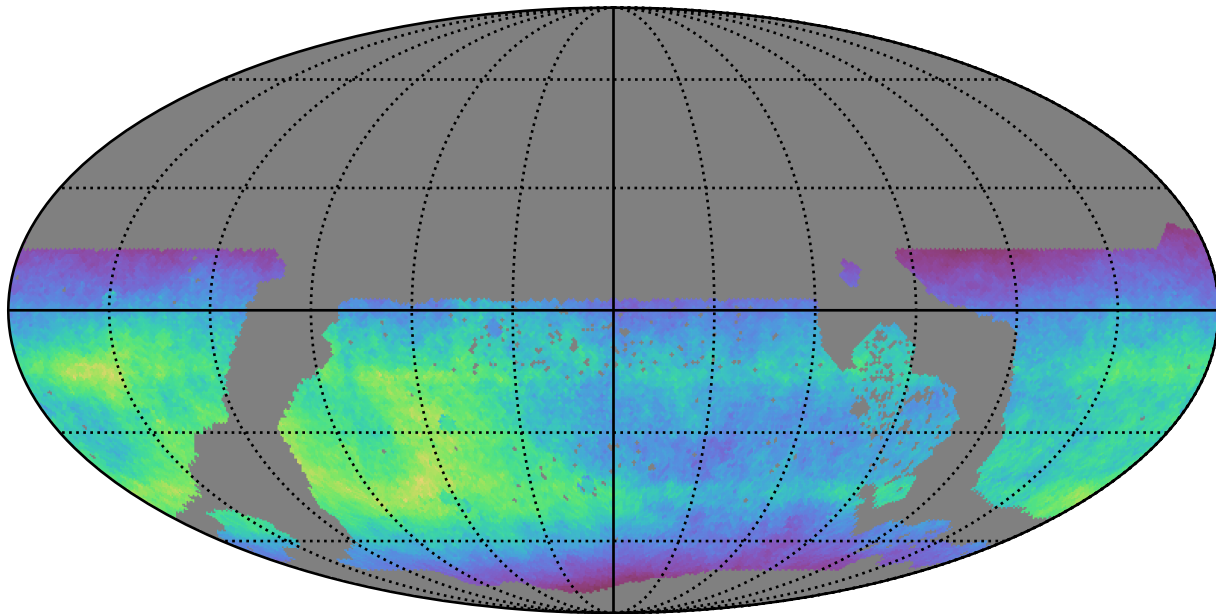
too_elab_r8_d2_giz_v3.4_10yrs WFD i band: Normalized Teff
