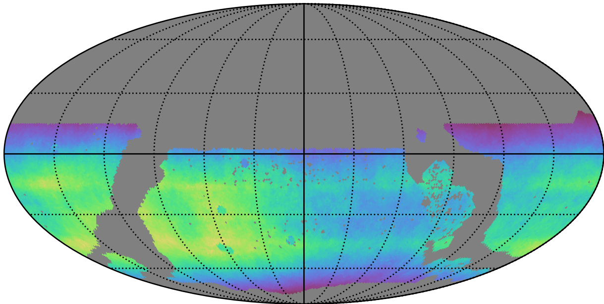
too_elab_r8_d2_giz_v3.4_10yrs WFD all bands: Normalized Teff
