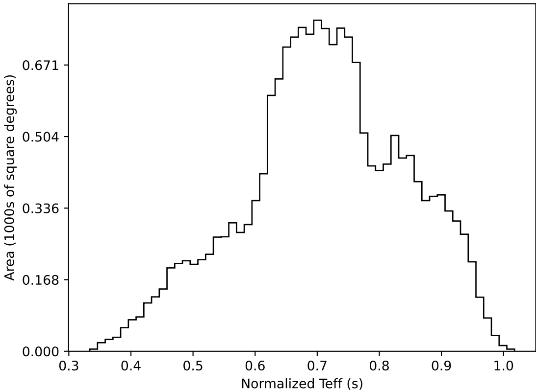
too_elab_r8_d2_giz_v3.4_10yrs WFD all bands: Normalized Teff
