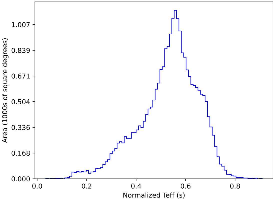
too_elab_r8_d2_giz_v3.4_10yrs All sky y band: Normalized Teff
