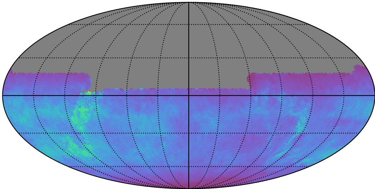
too_elab_r8_d2_giz_v3.4_10yrs All sky u band: Normalized Teff
