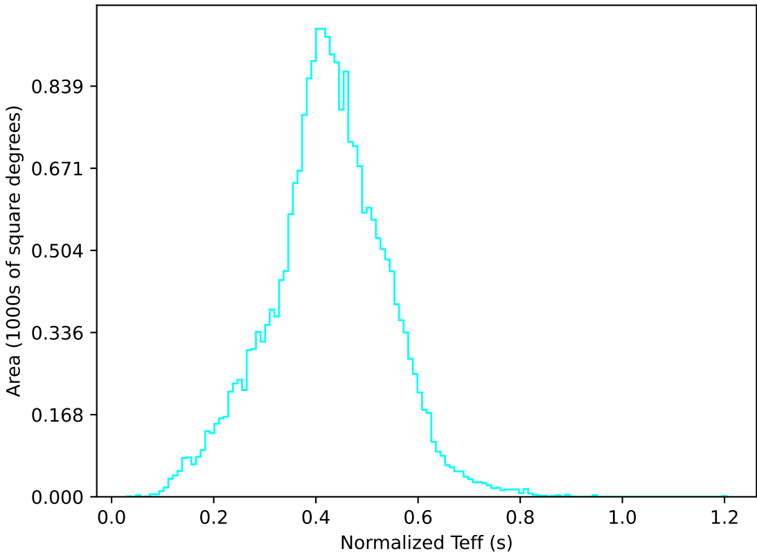
too_elab_r8_d2_giz_v3.4_10yrs All sky u band: Normalized Teff
