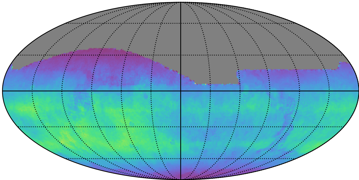
too_elab_r8_d2_giz_v3.4_10yrs All sky i band: Normalized Teff
