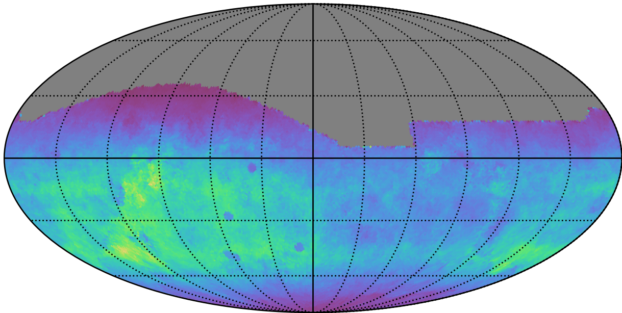
too_elab_r8_d2_giz_v3.4_10yrs All sky g band: Normalized Teff
