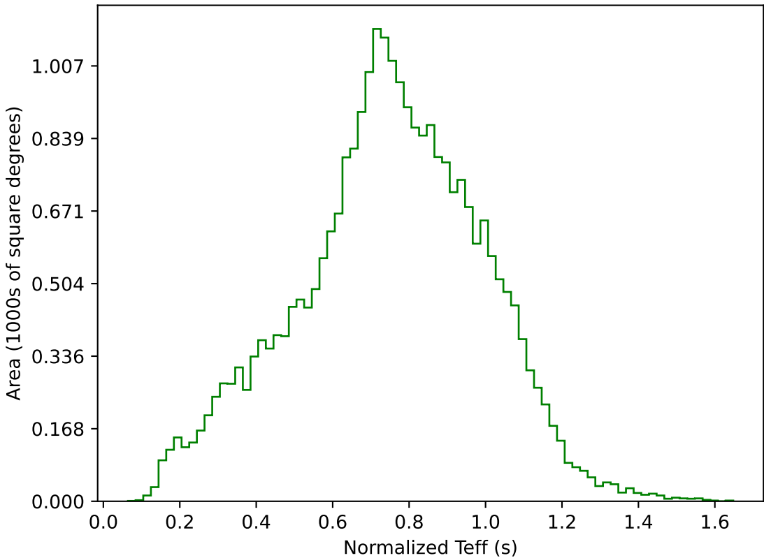
too_elab_r8_d2_giz_v3.4_10yrs All sky g band: Normalized Teff
