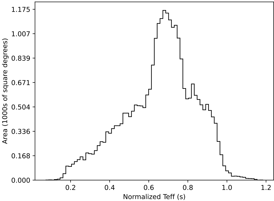
too_elab_r8_d2_giz_v3.4_10yrs All sky all bands: Normalized Teff
