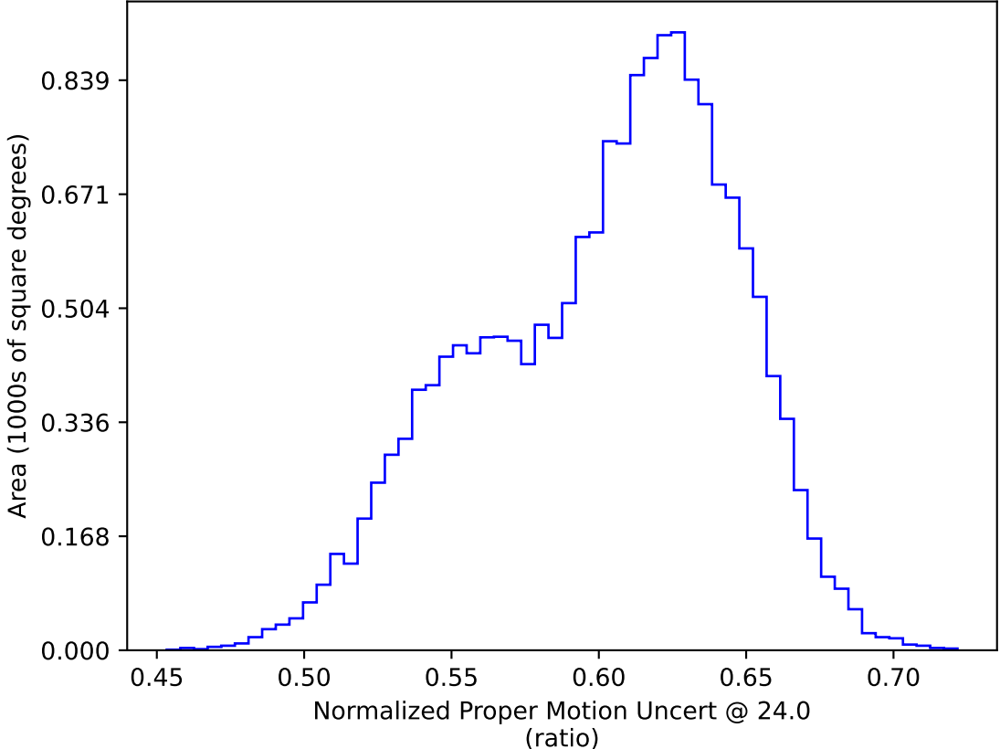
too_elab_r8_d2_giz_v3.4_10yrs WFD: Normalized Proper Motion Uncert @ 24.0
