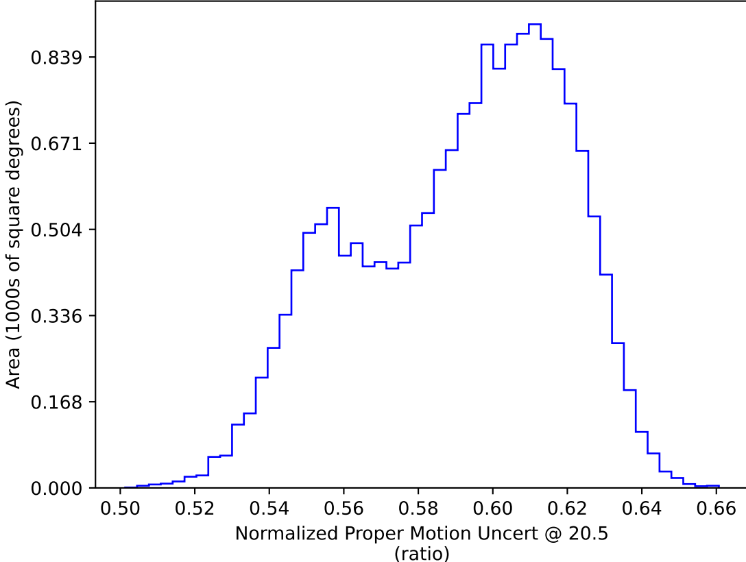
too_elab_r8_d2_giz_v3.4_10yrs WFD: Normalized Proper Motion Uncert @ 20.5
