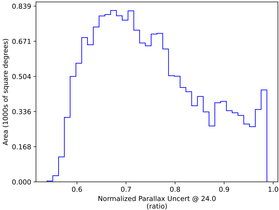
too_elab_r8_d2_giz_v3.4_10yrs WFD: Normalized Parallax Uncert @ 24.0
