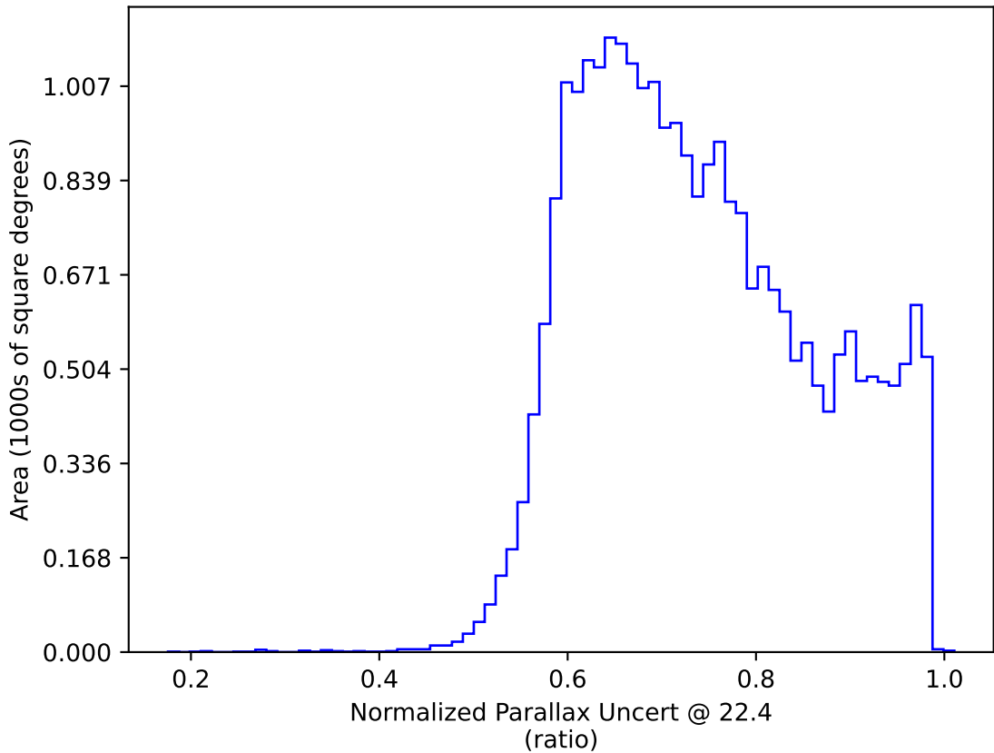
too_elab_r8_d2_giz_v3.4_10yrs All sky: Normalized Parallax Uncert @ 22.4
