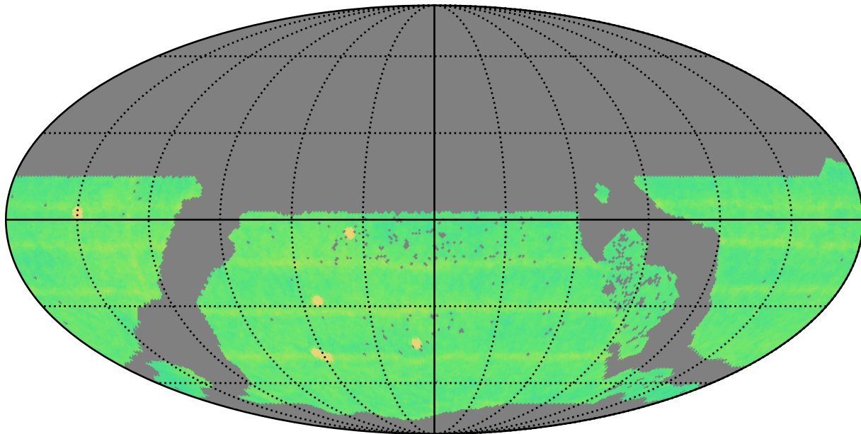
too_elab_r8_d2_giz_v3.4_10yrs WFD all bands: N Unique Nights
