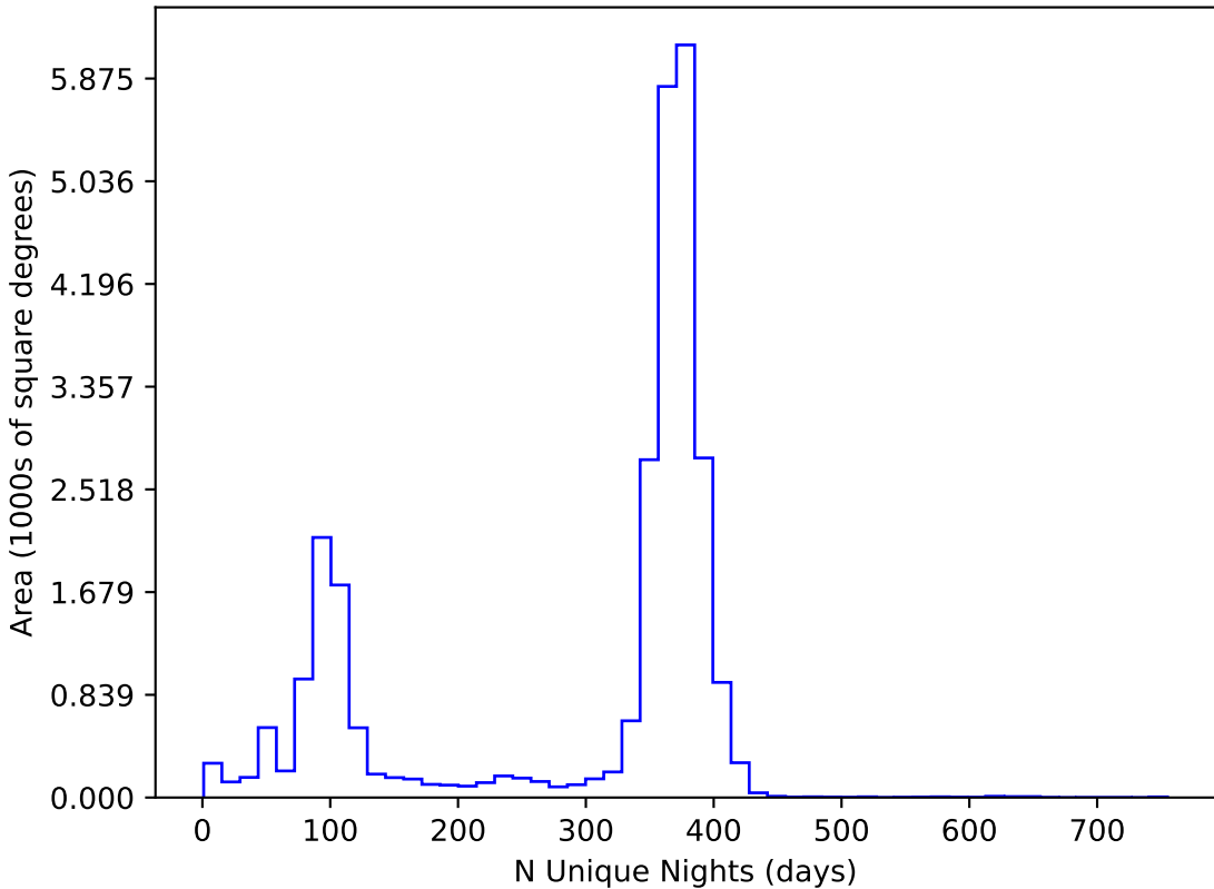
too_elab_r8_d2_giz_v3.4_10yrs All sky all bands: N Unique Nights
