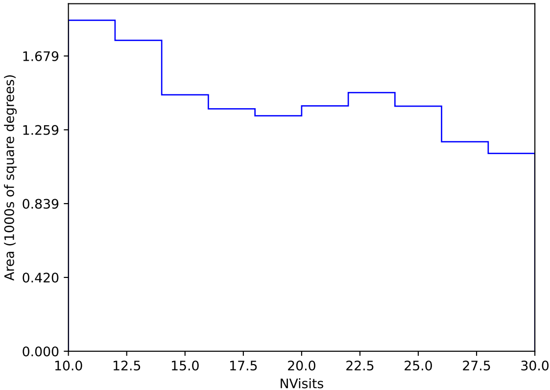
too_elab_r8_d2_giz_v3.4_10yrs Yr 3-4 y band: NVisits
