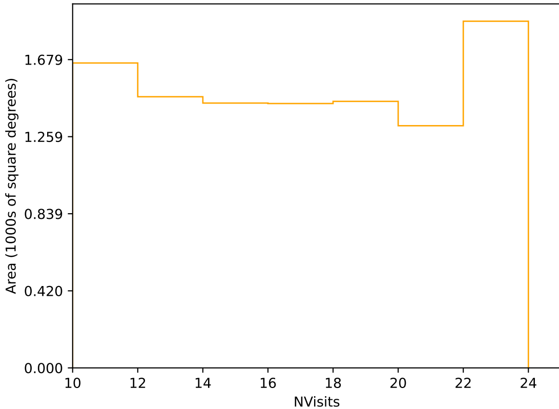
too_elab_r8_d2_giz_v3.4_10yrs Yr 3-4 r band: NVisits
