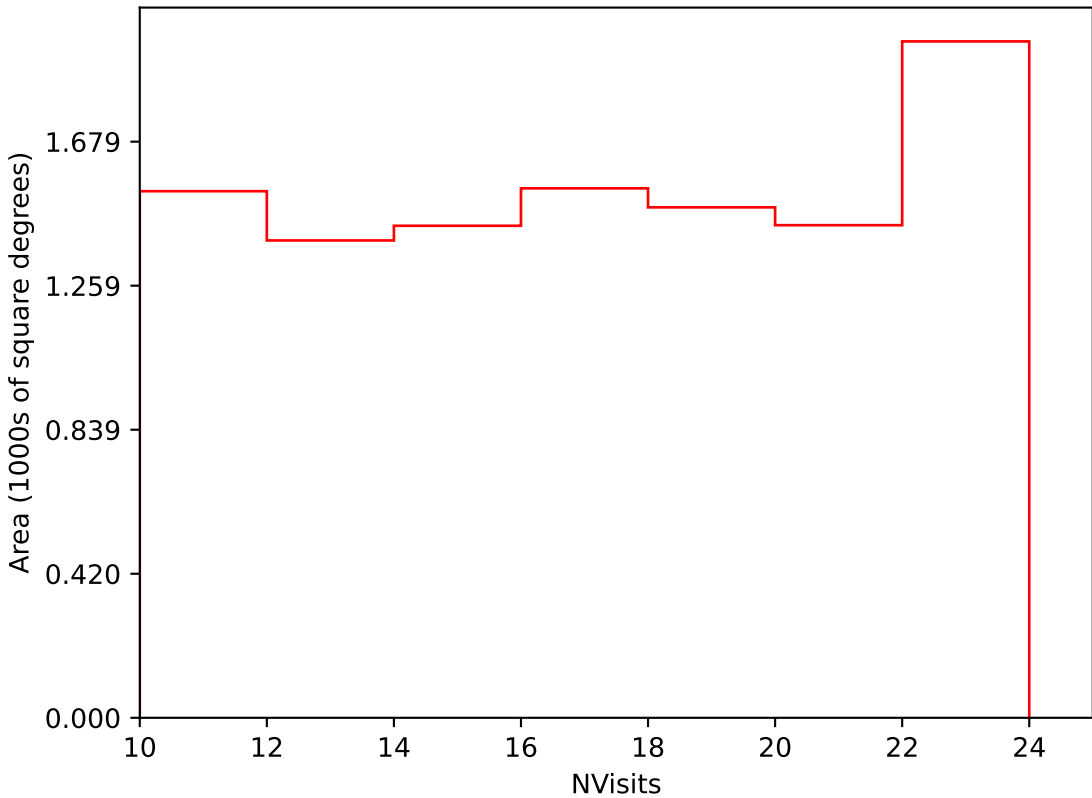
too_elab_r8_d2_giz_v3.4_10yrs Yr 3-4 i band: NVisits
