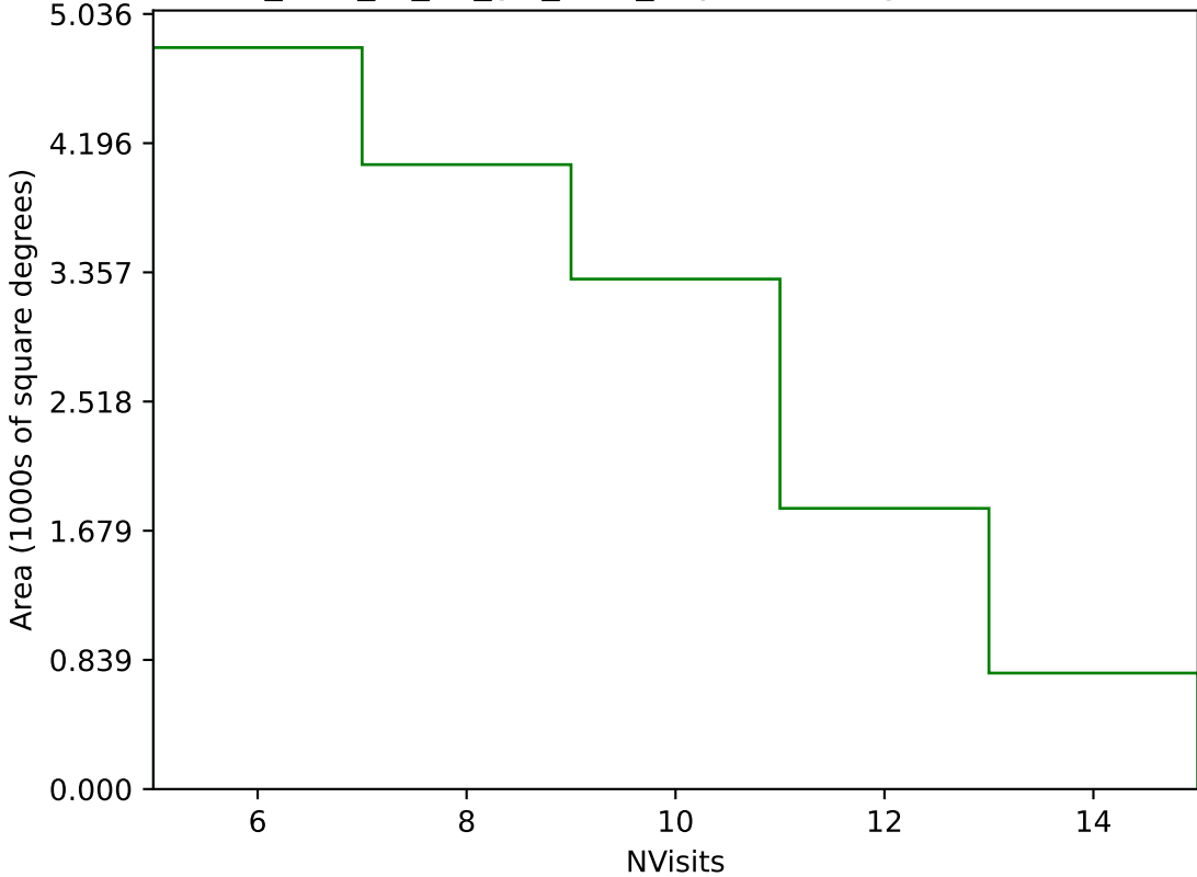
too_elab_r8_d2_giz_v3.4_10yrs Yr 3-4 g band: NVisits
