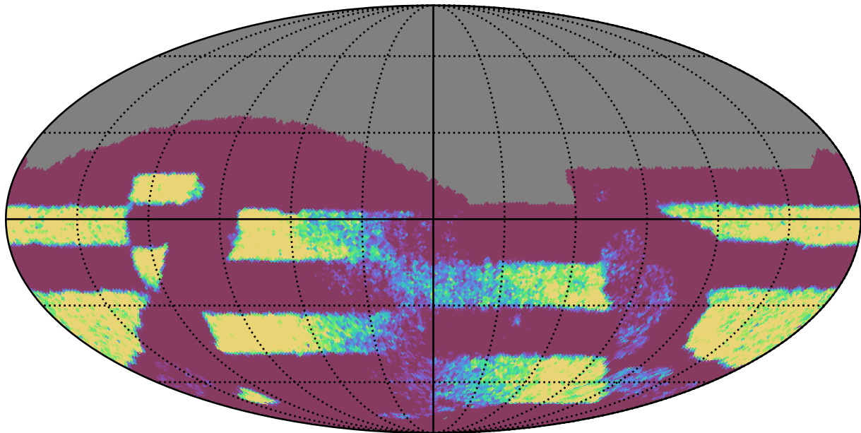
too_elab_r8_d2_giz_v3.4_10yrs Yr 3-4 all bands: NVisits
