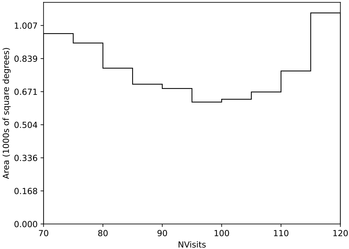
too_elab_r8_d2_giz_v3.4_10yrs Yr 3-4 all bands: NVisits
