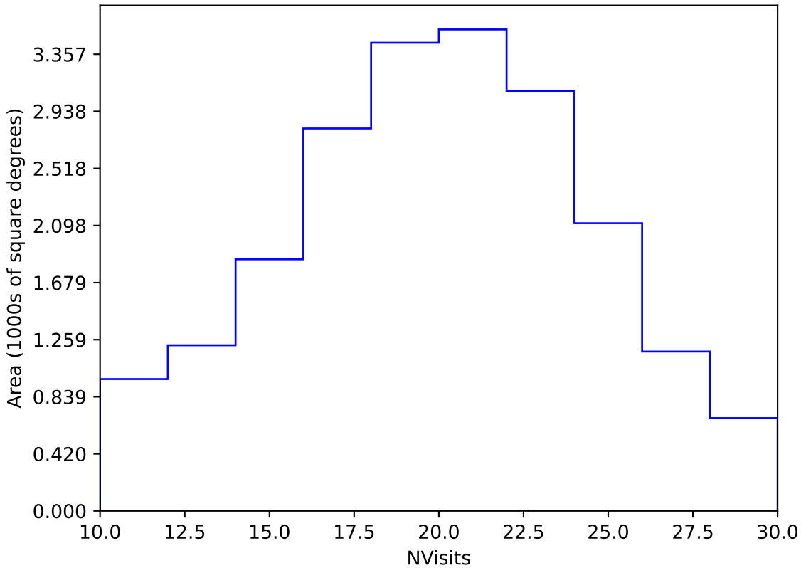
too_elab_r8_d2_giz_v3.4_10yrs Yr 1 y band: NVisits
