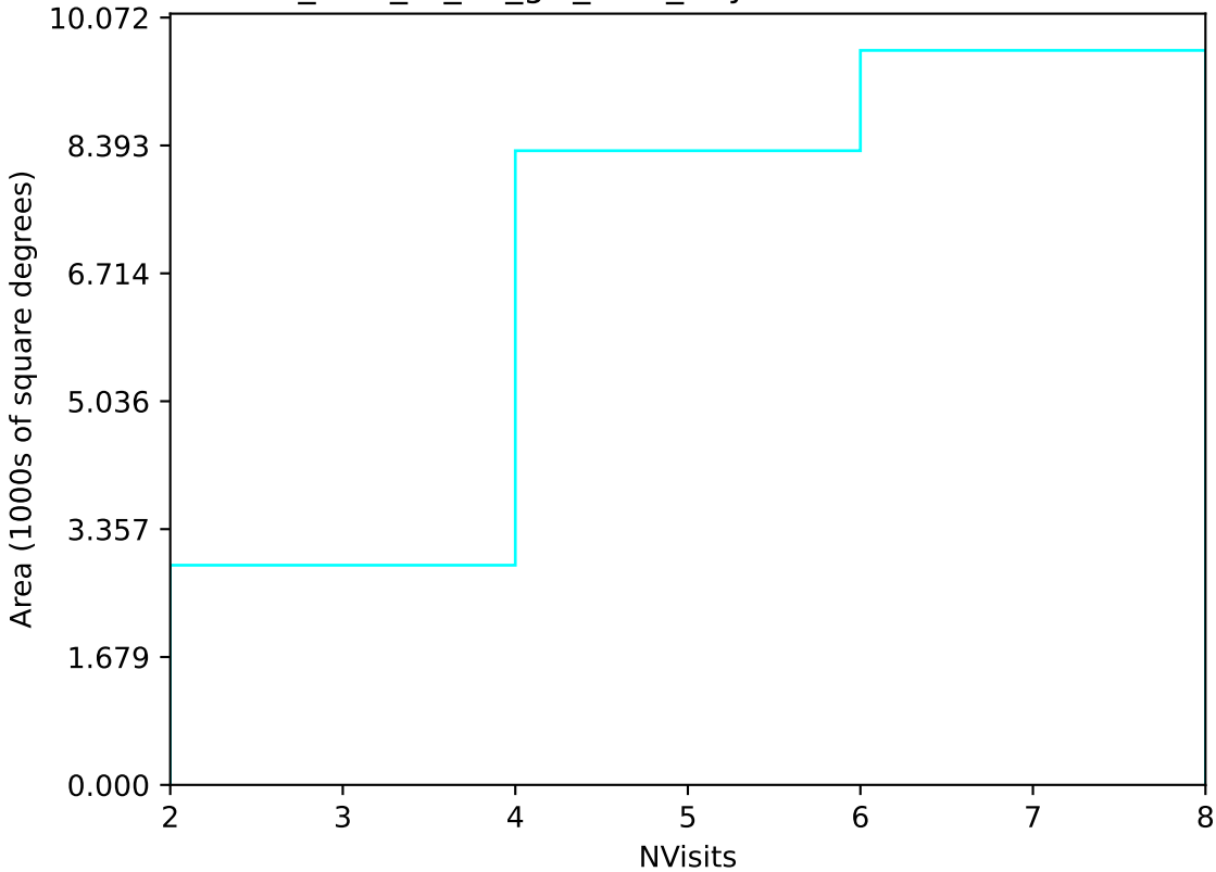
too_elab_r8_d2_giz_v3.4_10yrs Yr 1 u band: NVisits
