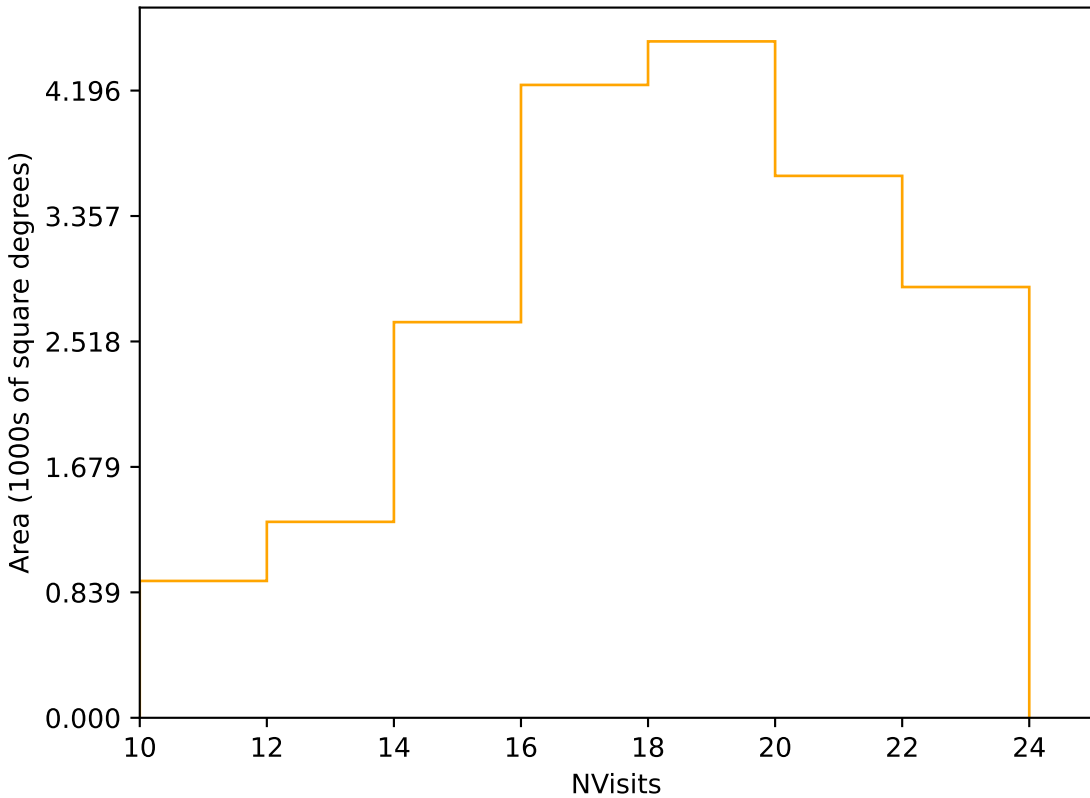
too_elab_r8_d2_giz_v3.4_10yrs Yr 1 r band: NVisits
