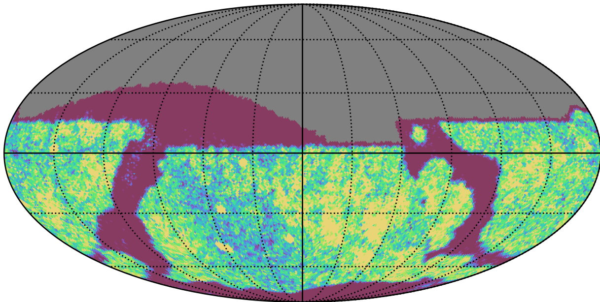
too_elab_r8_d2_giz_v3.4_10yrs Yr 1 i band: NVisits
