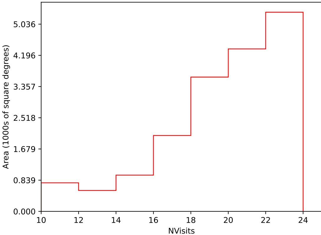
too_elab_r8_d2_giz_v3.4_10yrs Yr 1 i band: NVisits
