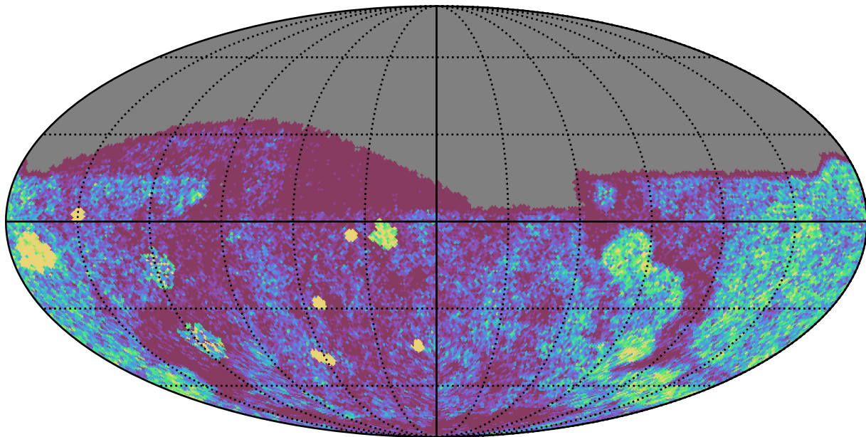
too_elab_r8_d2_giz_v3.4_10yrs Yr 1 g band: NVisits
