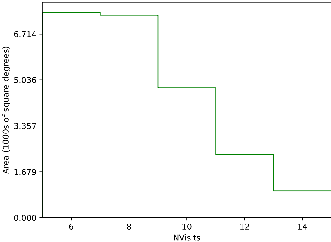
too_elab_r8_d2_giz_v3.4_10yrs Yr 1 g band: NVisits
