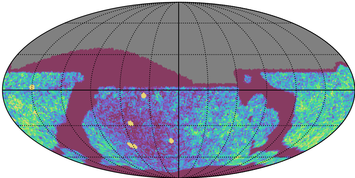
too_elab_r8_d2_giz_v3.4_10yrs Yr 1 all bands: NVisits
