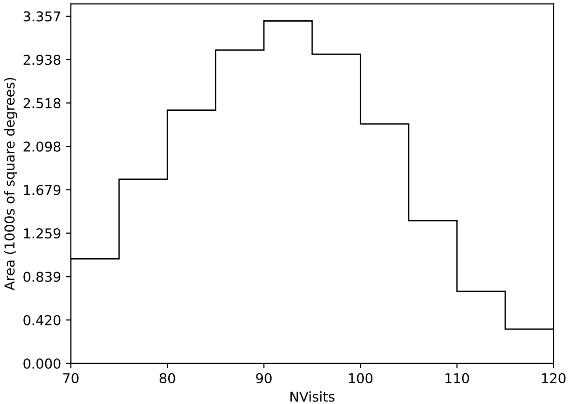
too_elab_r8_d2_giz_v3.4_10yrs Yr 1 all bands: NVisits
