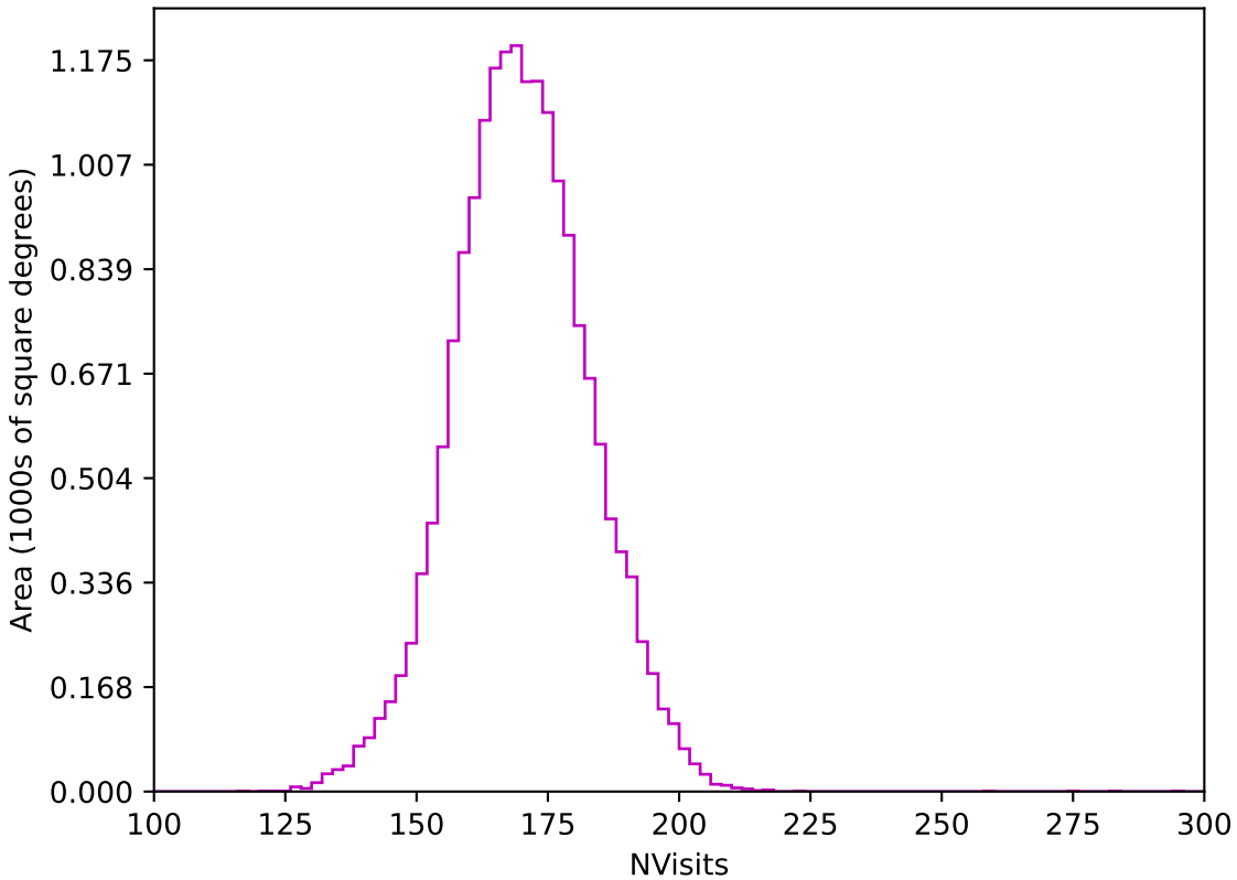
too_elab_r8_d2_giz_v3.4_10yrs WFD z band: NVisits
