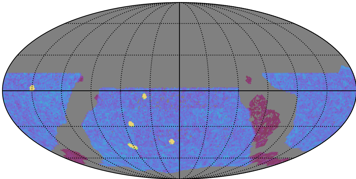
too_elab_r8_d2_giz_v3.4_10yrs WFD y band: NVisits
