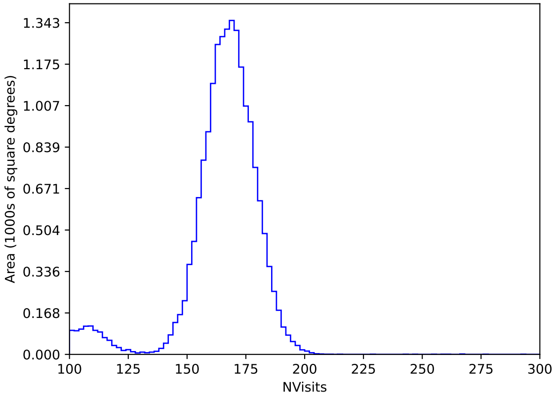
too_elab_r8_d2_giz_v3.4_10yrs WFD y band: NVisits
