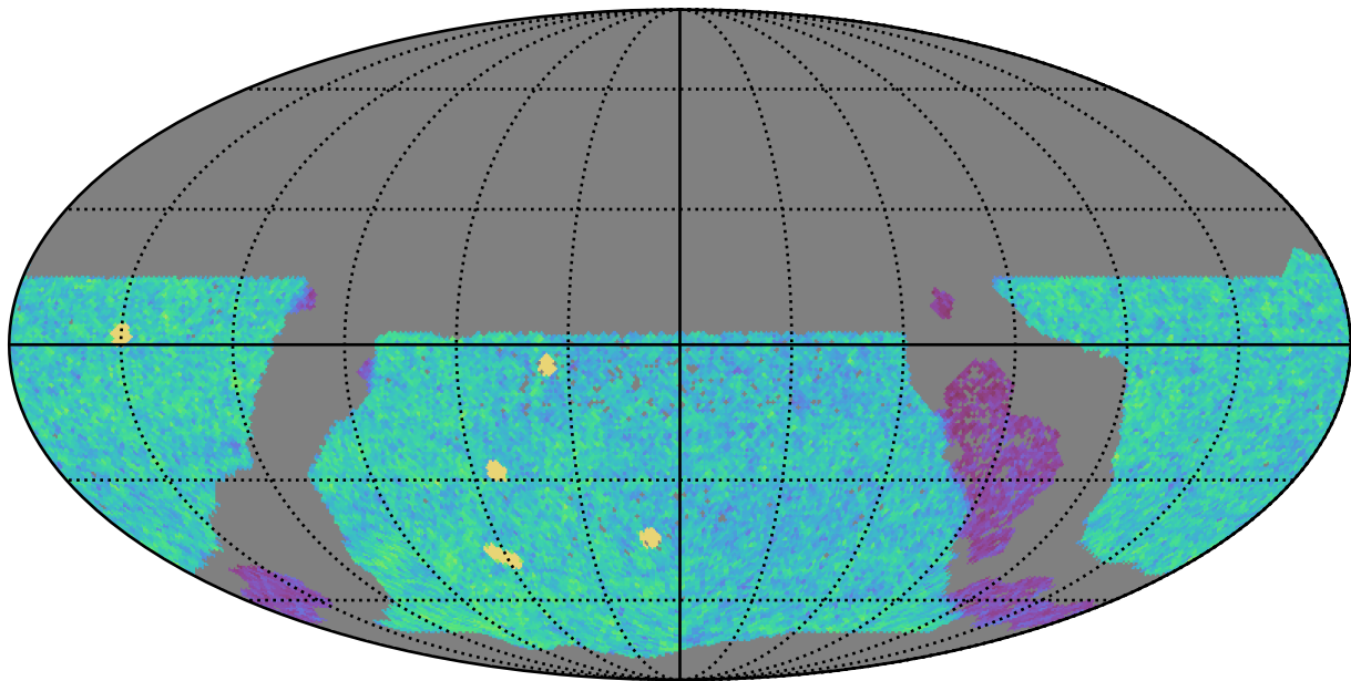
too_elab_r8_d2_giz_v3.4_10yrs WFD u band: NVisits
