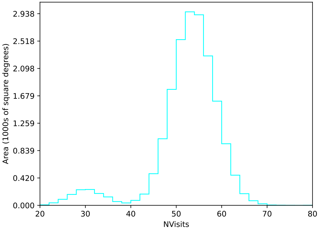
too_elab_r8_d2_giz_v3.4_10yrs WFD u band: NVisits
