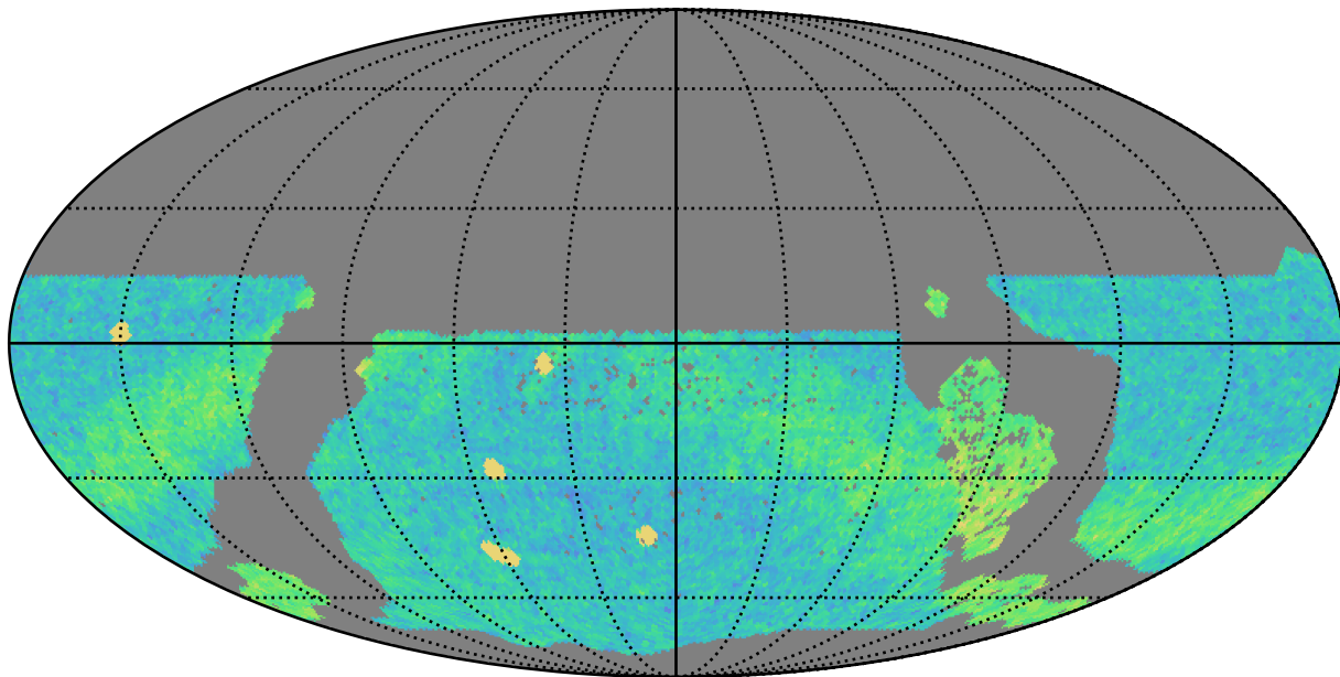
too_elab_r8_d2_giz_v3.4_10yrs WFD r band: NVisits
