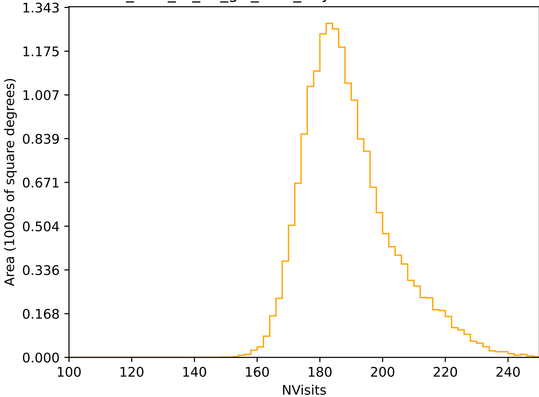
too_elab_r8_d2_giz_v3.4_10yrs WFD r band: NVisits
