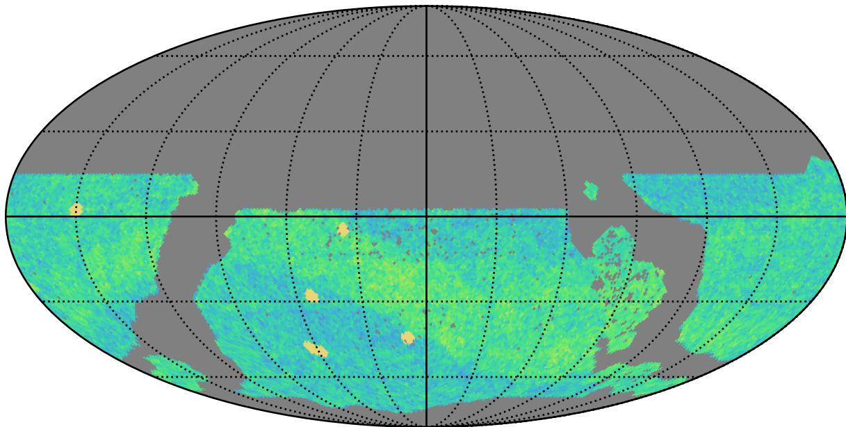
too_elab_r8_d2_giz_v3.4_10yrs WFD i band: NVisits
