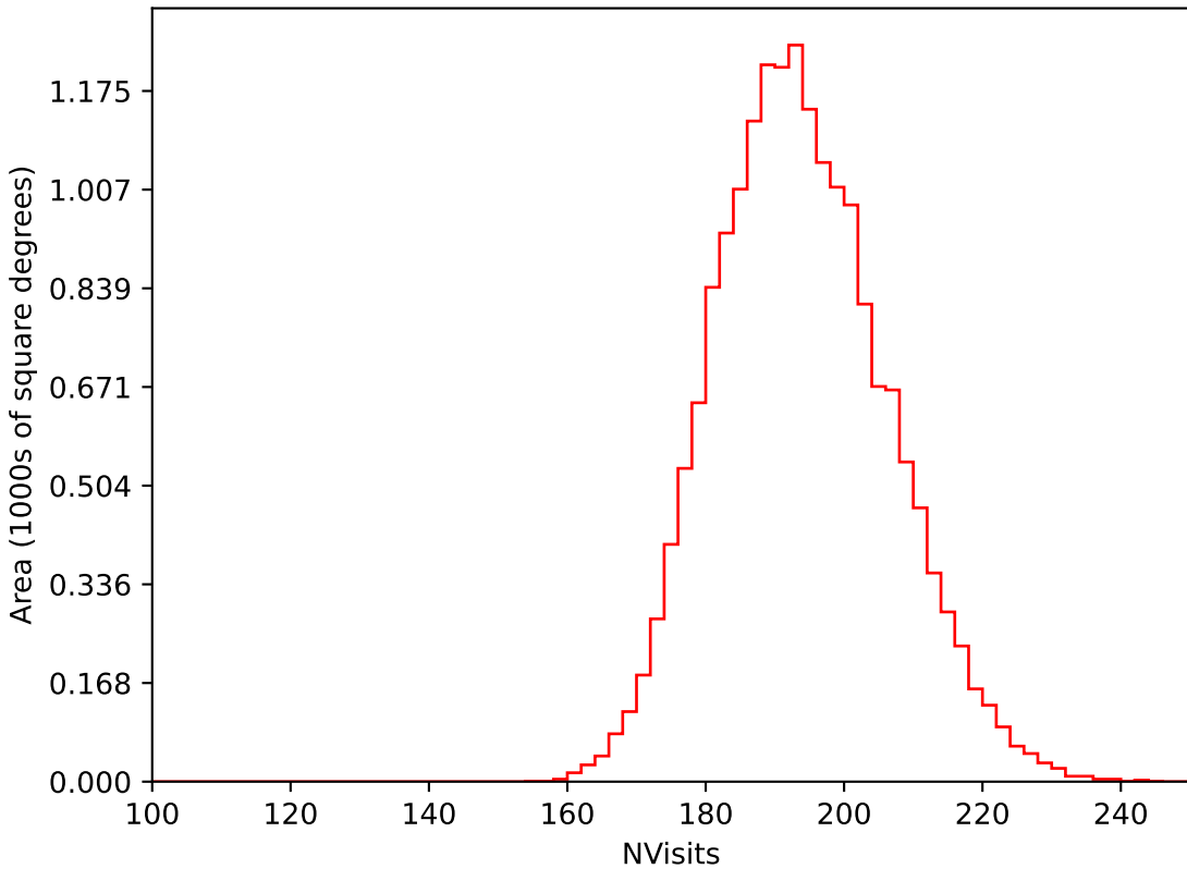
too_elab_r8_d2_giz_v3.4_10yrs WFD i band: NVisits
