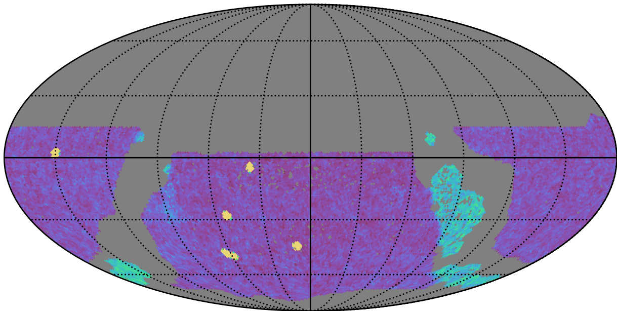
too_elab_r8_d2_giz_v3.4_10yrs WFD g band: NVisits
