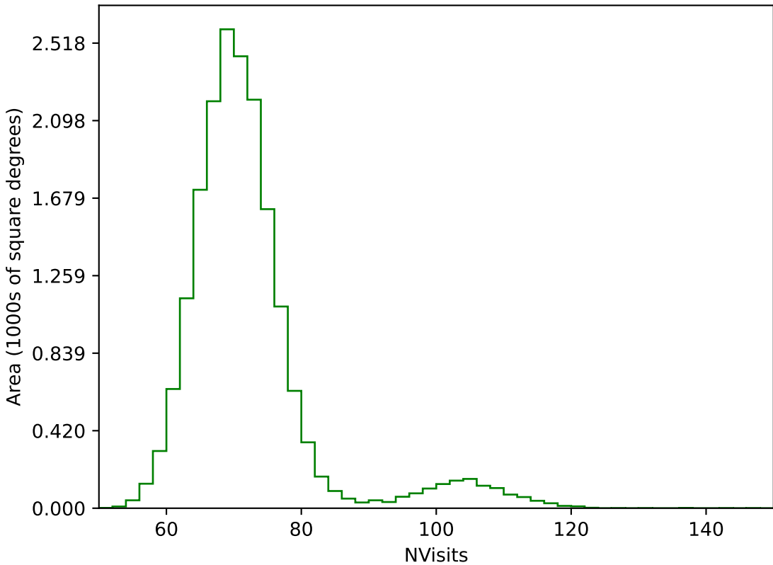
too_elab_r8_d2_giz_v3.4_10yrs WFD g band: NVisits
