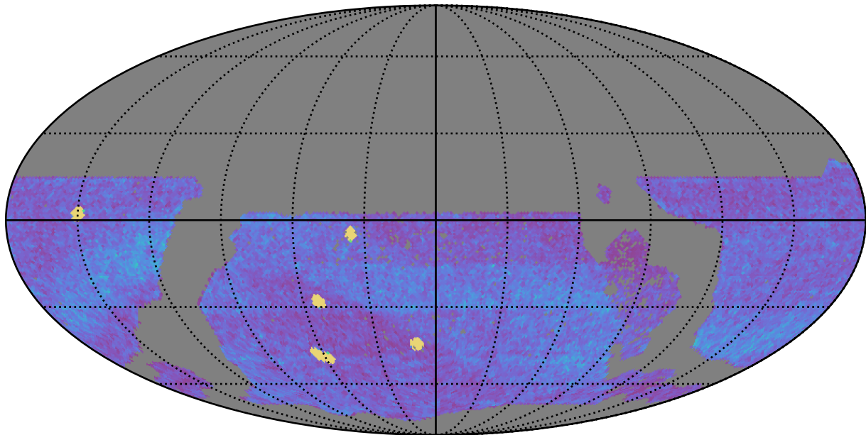
too_elab_r8_d2_giz_v3.4_10yrs WFD all bands: NVisits
