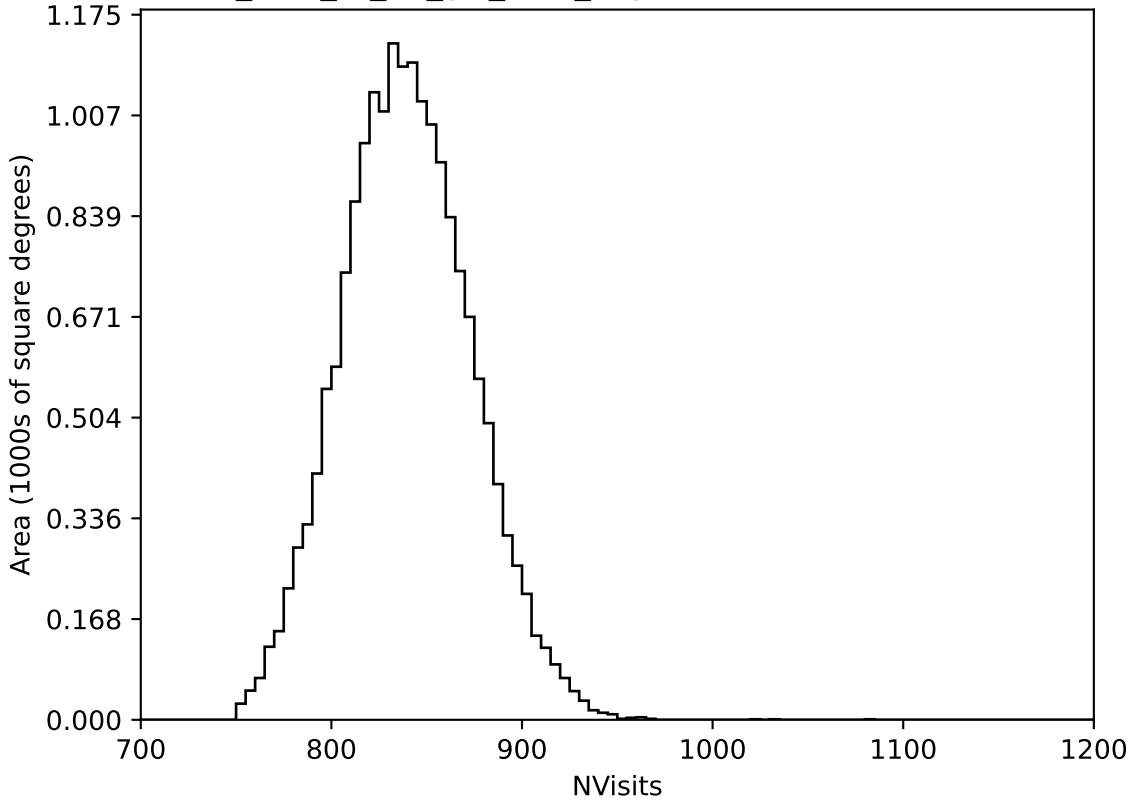
too_elab_r8_d2_giz_v3.4_10yrs WFD all bands: NVisits
