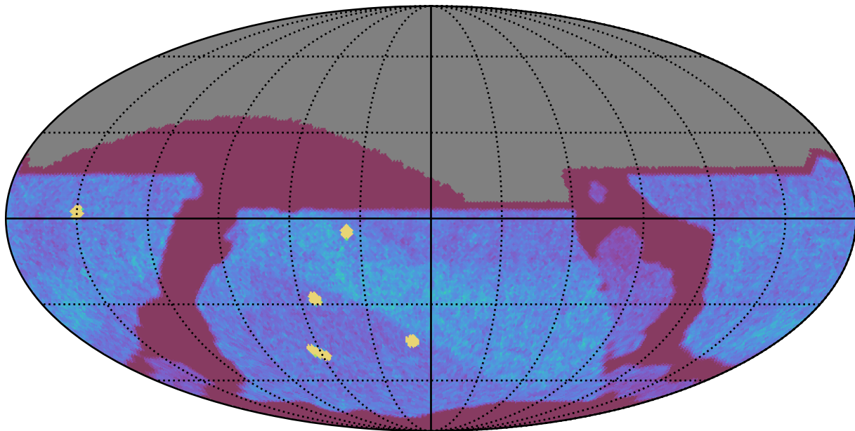
too_elab_r8_d2_giz_v3.4_10yrs All sky z band: NVisits
