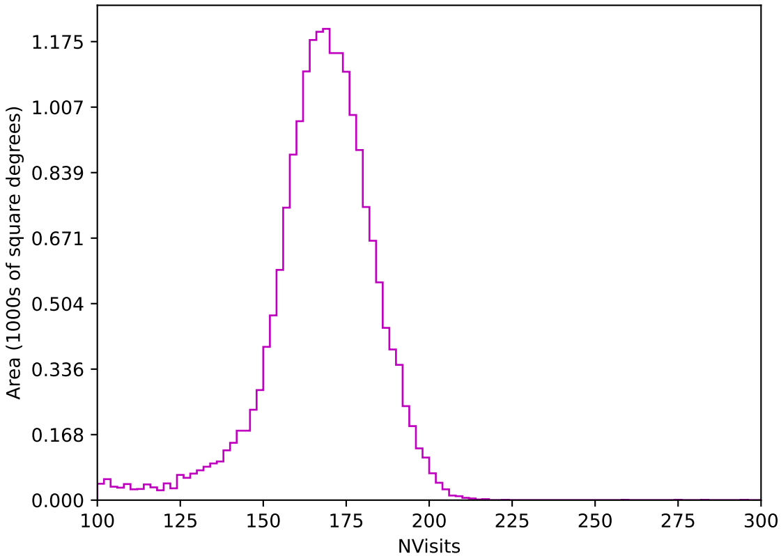
too_elab_r8_d2_giz_v3.4_10yrs All sky z band: NVisits
