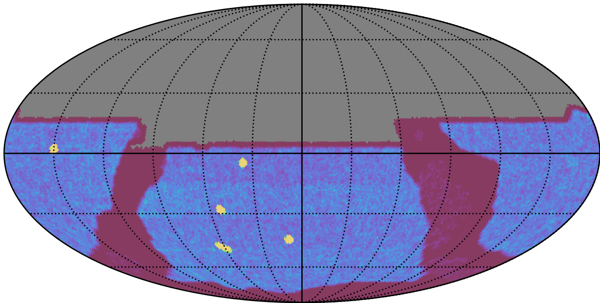
too_elab_r8_d2_giz_v3.4_10yrs All sky y band: NVisits
