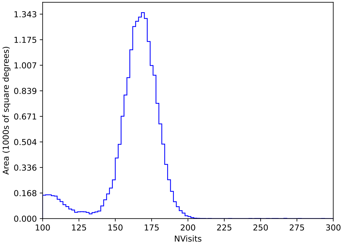
too_elab_r8_d2_giz_v3.4_10yrs All sky y band: NVisits
