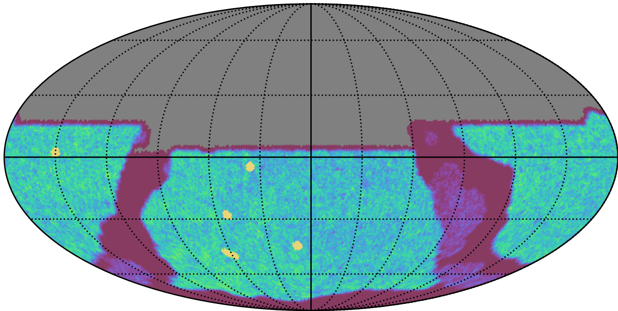
too_elab_r8_d2_giz_v3.4_10yrs All sky u band: NVisits
